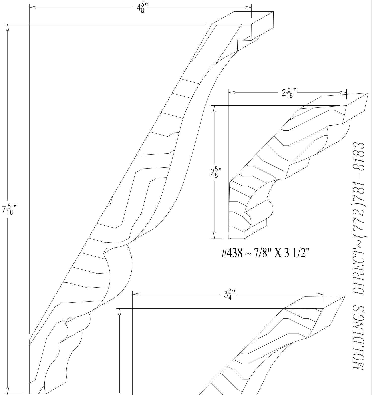
#436 ~ 7/8" X 8 1/2"
