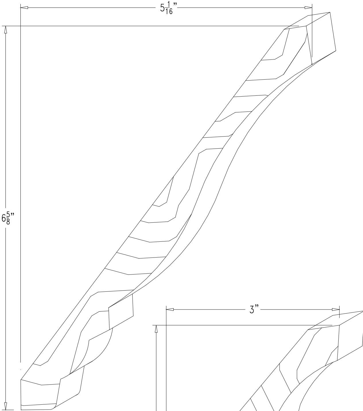
#401 ~ 3/4" X 8 1/4"
