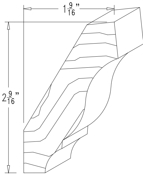
#405 ~ 3/4" X 3"
