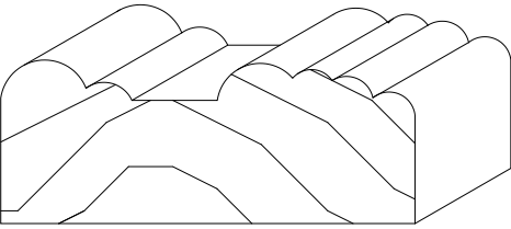
#539 ~ 3/4" X 1 7/8"
