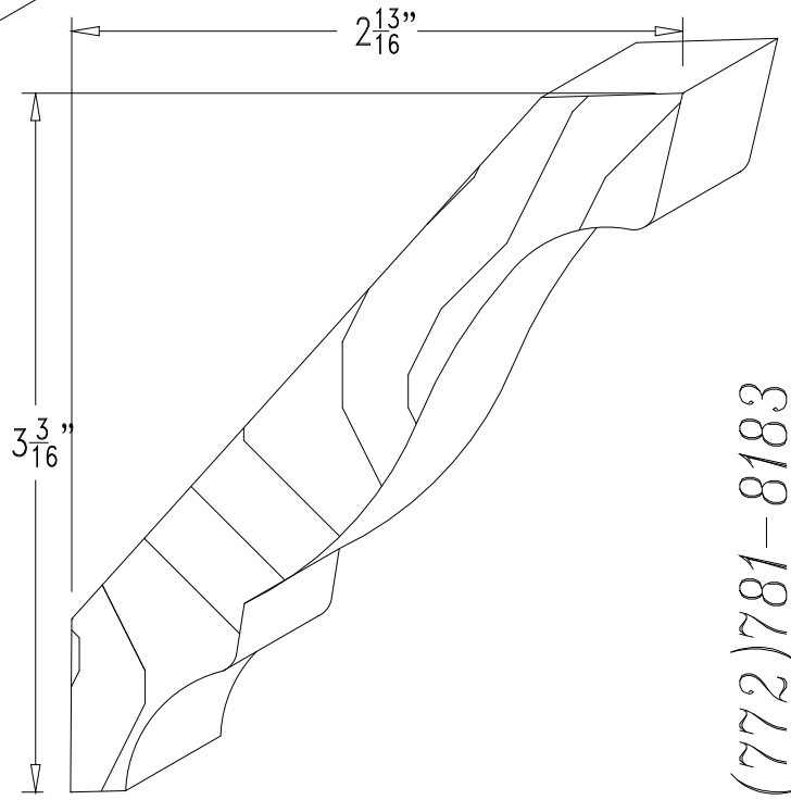
#404 ~ 3/4" X 4 1/4"
