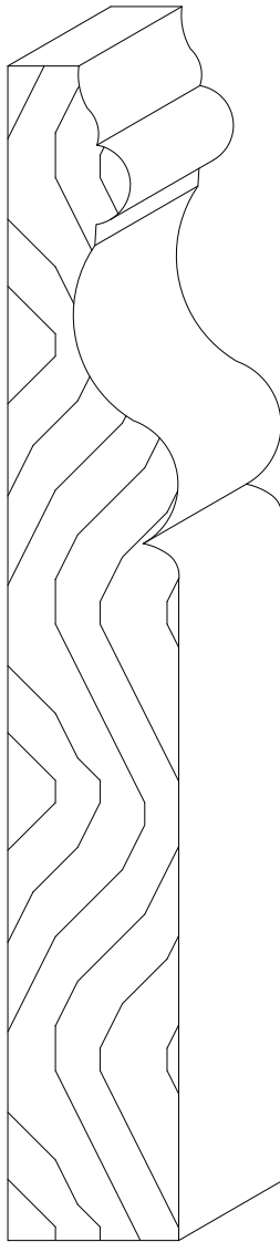
#220 ~ 3/4" X 5 1/4"
