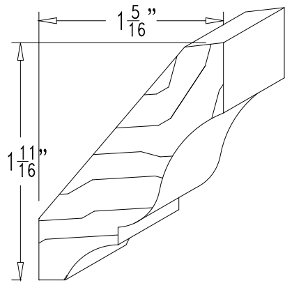
#434 ~ 5/8" X 2 1/8"
