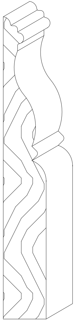
#209 ~ 3/4" X 5 1/4"-7 1/4"
