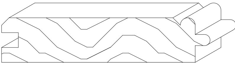
#567 ~ 3/4" X 3 1/2"
