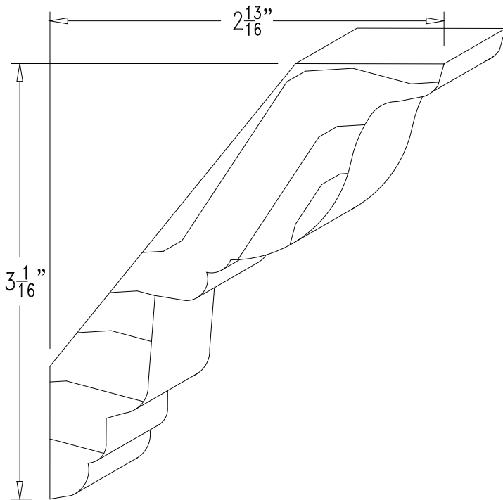
#423 ~ 7/8" X 4 3/16"
