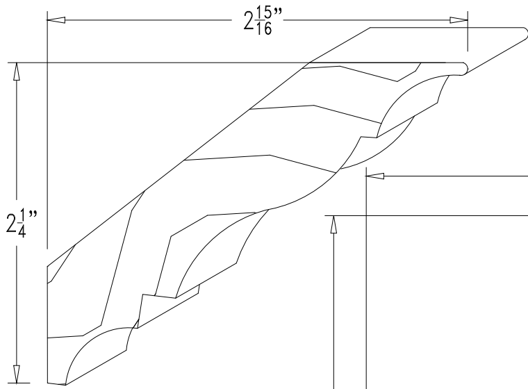
#432 ~ 3/4" X 3 3/4"
