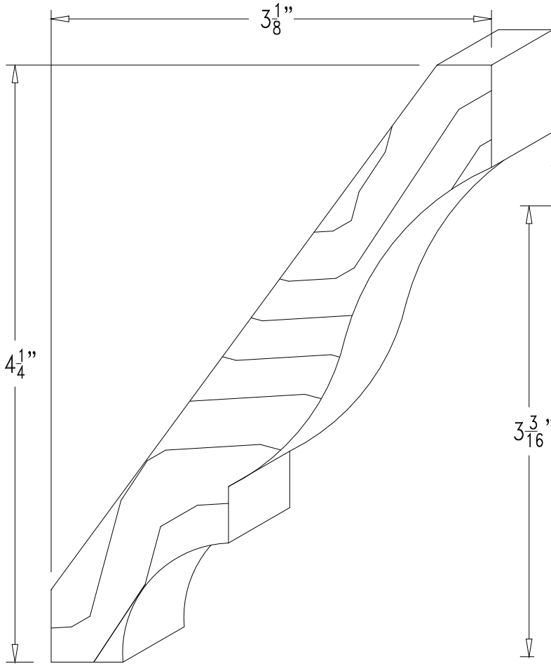
#403 ~ 3/4" X 5 1/4"
