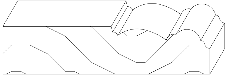
#105 ~ 13/16" X 3 1/2" MATCHES BASE #205
