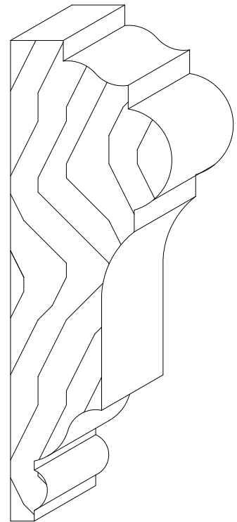
#312 ~ 1 1/8" X 3 3/8"
