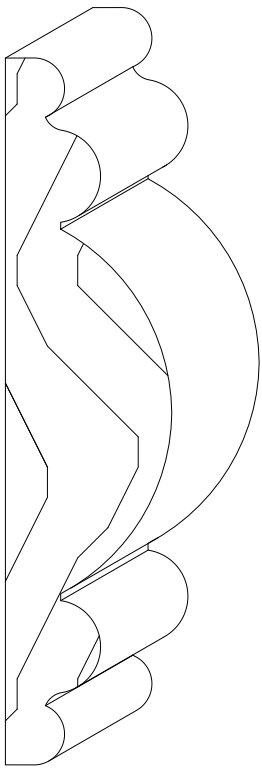
#301 ~ 13/16" X 3 1/2"
