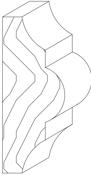
#308 ~ 1" X 2 1/2"
