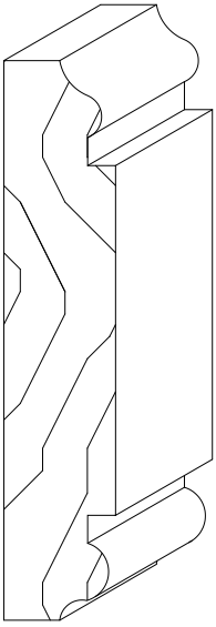
#307 ~ 1/2" X 2 1/2"
