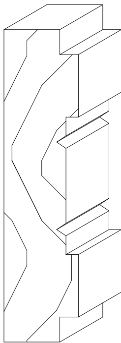
#328 ~ 3/4" X 3 1/8"
