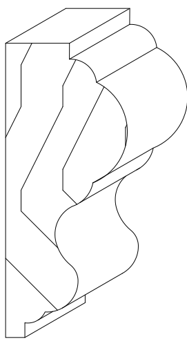
#305 ~ 7/8" X 2 1/8"
