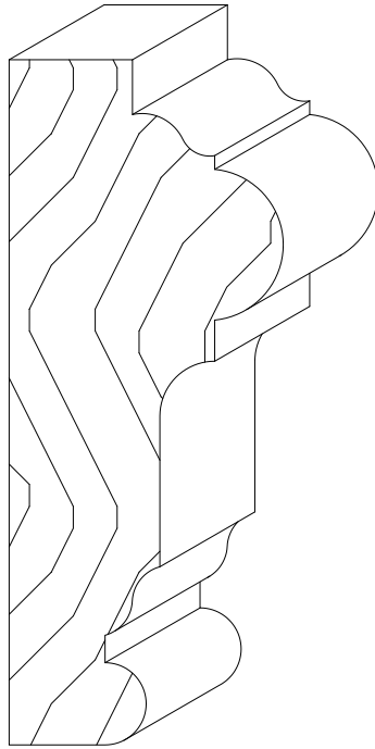
#314 ~ 1 1/4" X 3 1/8"
